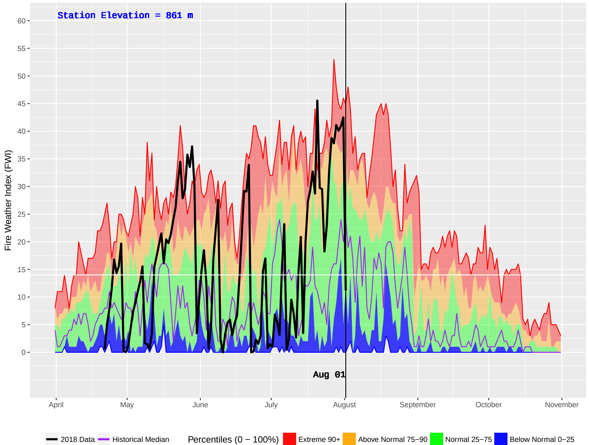
BLAEBERRY (866) : Historical (2004–2016) and Current (2018) Daily Fire Weather Index (FWI)
