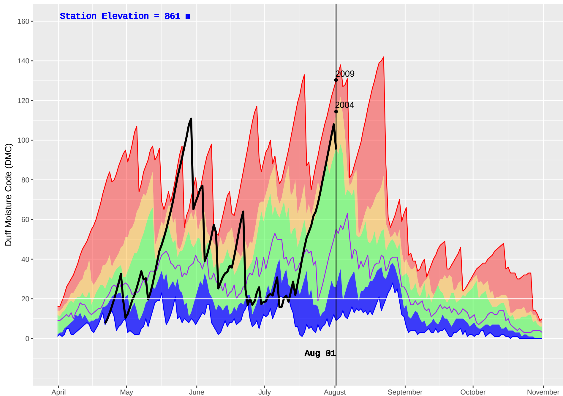
BLAEBERRY (866) : Historical (2004–2016) and Current (2018) Daily Duff Moisture Code (DMC)
