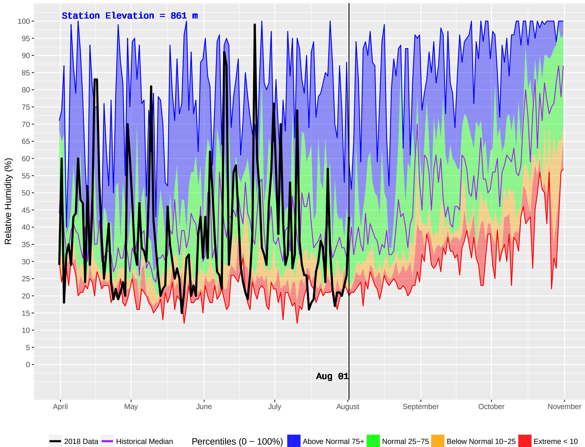
BLAEBERRY (866) : Historical (2004–2016) and Current (2018) Daily Relative Humidity
